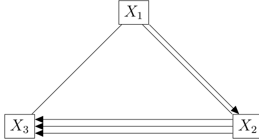
Figure 4: Ranking problem of Example 4
