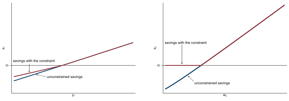
(a) Optimal savings in period 1; negative values indicate borrowing
