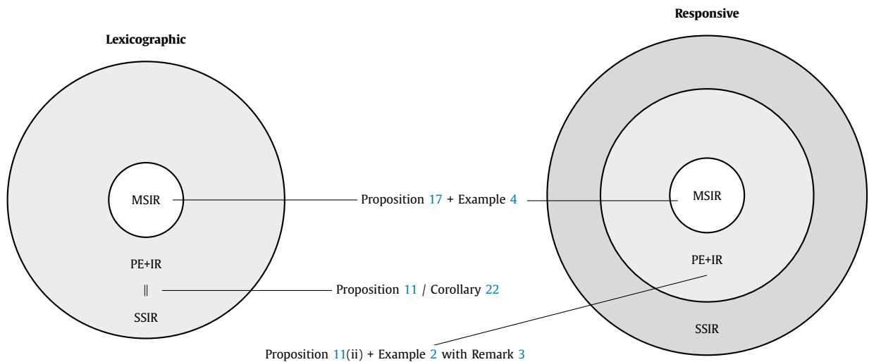
Fig. 2. Venn diagrams. Fix preferences P . Let PE+IR denote the set of Pareto-efficient and individually rational circulations at P . Let SSIR ( MSIR ) denote the set of circulations obtained by applying Single-Serial-IR (Multiple-Serial-IR) rules to \succ^P . The examples show that the set inclusion can be strict.
