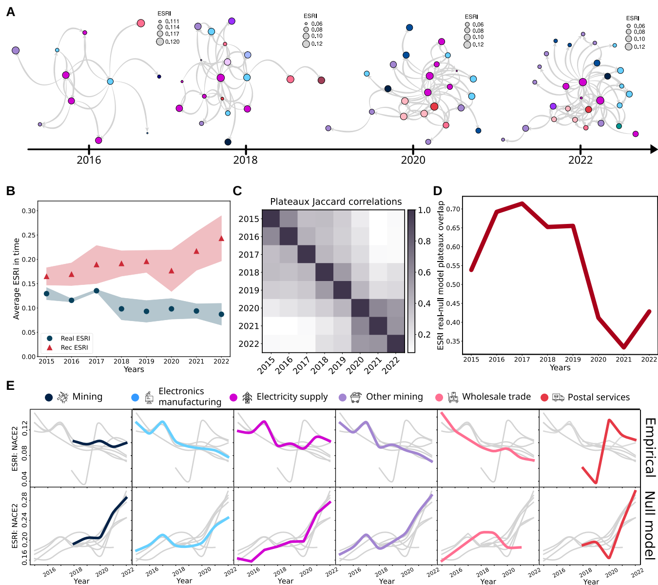
Figure 4 ESRI plateaux analysis. A) Representation of the empirical network among plateau firms, with node size proportional to ESRI values and color identifying the NACE2 sector. B) Average ESRI for plateaux firms, displaying the same trend observed for the whole networks. C) Matrix of Jaccard indices quantifying the overlap among the sets of empirical plateaux firms between different years. D) Time evolution of the Jaccard coefficient of plateau firms sets between empirical vs. model networks in the same year. E) Evolution of empirical (top panels) and null (bottom panels) ESRI values, for firms appearing more than 3 years in the plateaux, grouped by NACE2 sectors. Each panel highlights the evolution of a single sector (the other sectors are displayed in gray).
